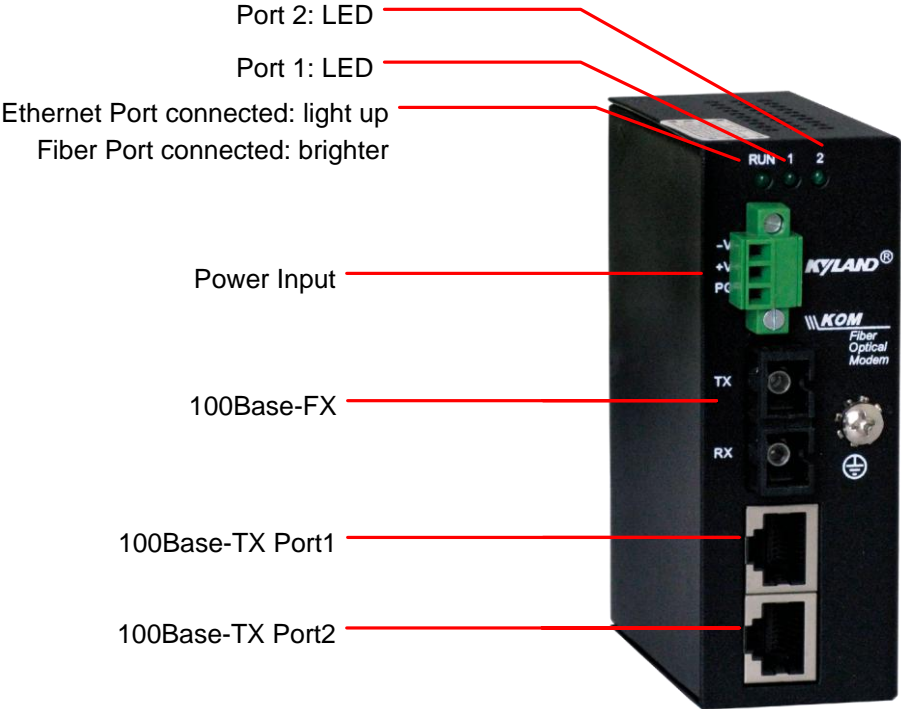
Figure1-Front Pannel
