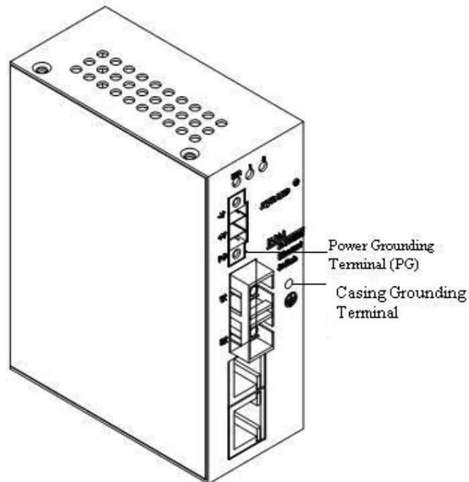
Figure 4: Device grounding
